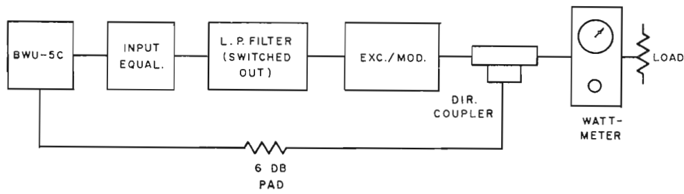
FIG. 5. Response analyzer setup for tuning of UHF exciter with video modulation.
