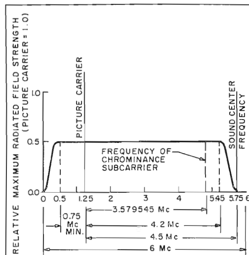
FIG. 9. Idealized vestigial sideband picture transmission amplitude characteristic.
