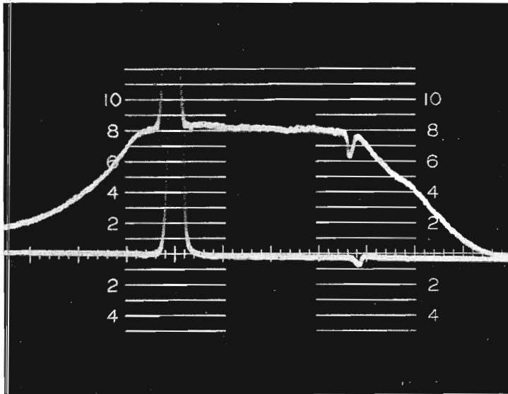
(b) Modulated amplifier output into dummy load.
