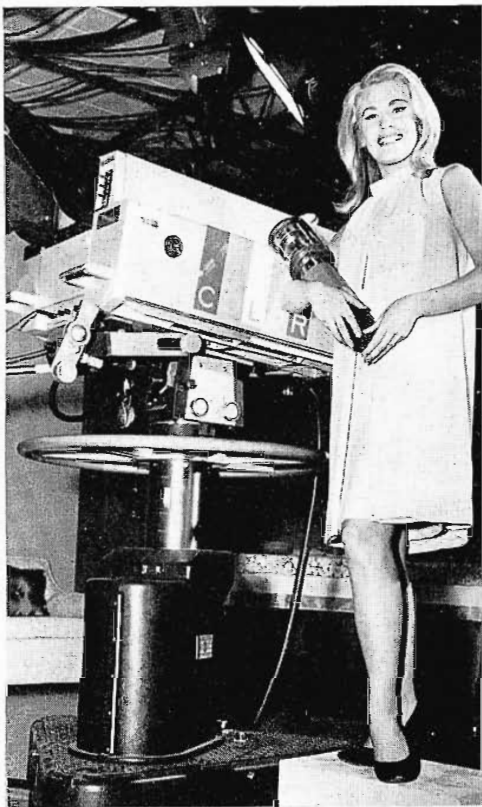
Donna Rae Wood smiles engagingly as she cradles No. 4536 like the newborn 4½-inch image orthicon that it is. New pickup tube that reduces signal-to-noise ratio made its debut in TK-42/43 cameras.
