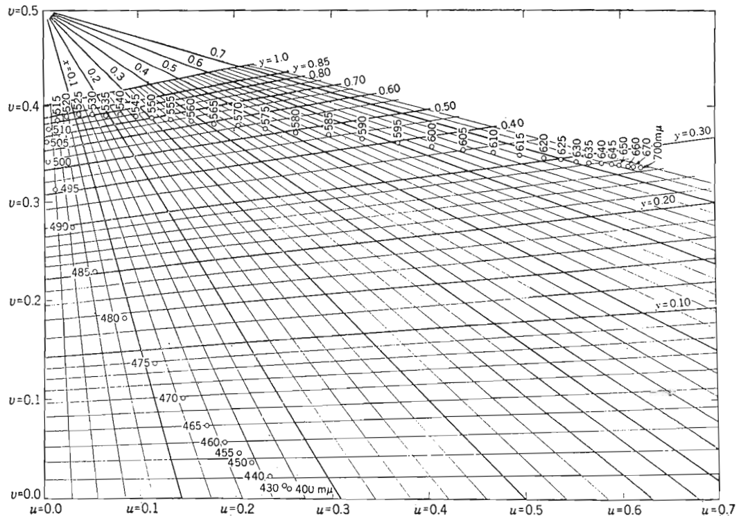
FIG. B1. Uniform Chromaticity Scale Diagram.
