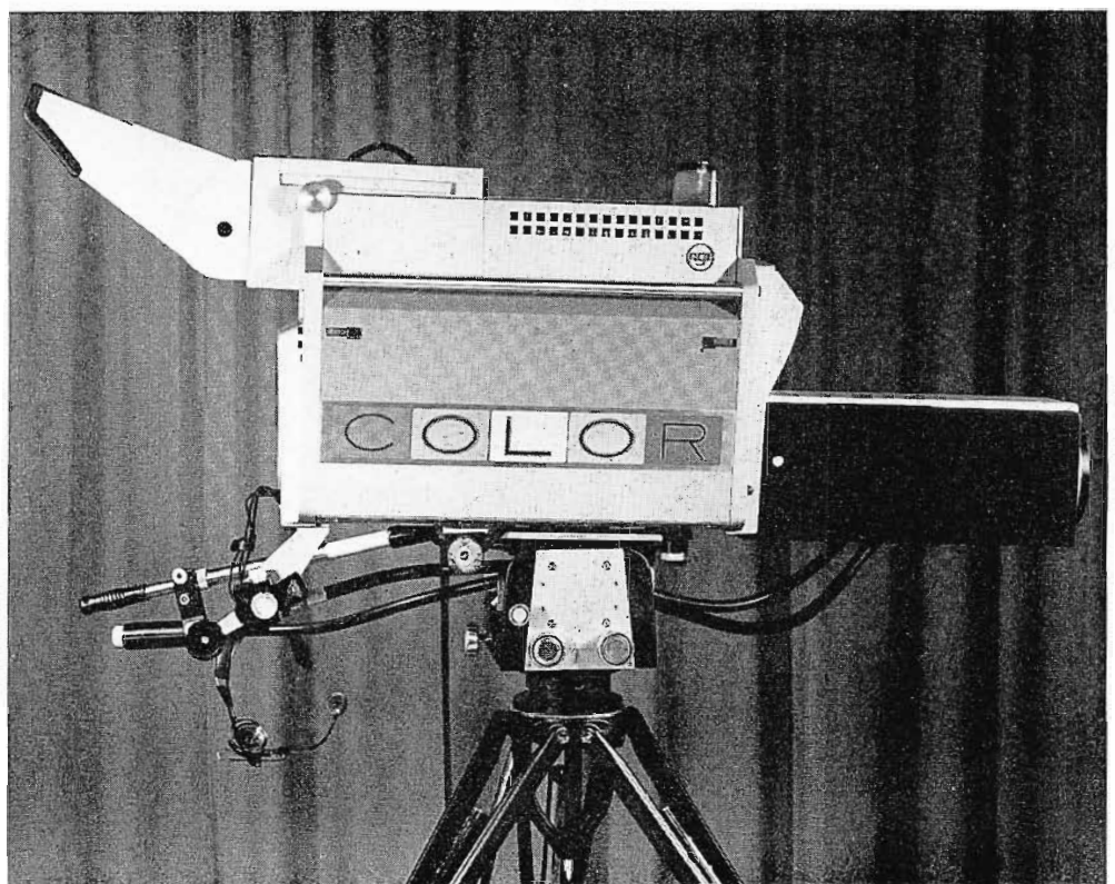
FIG. 5. Focus controls are grouped for easy operation by one hand. Viewfinder and zoom lens assembly are detachable from camera head for easy portability.
