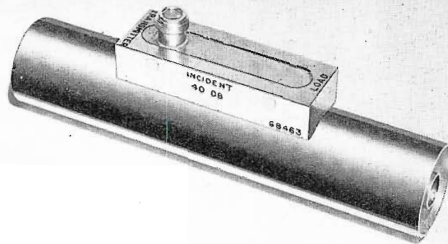
FIG. 6. VHF directional coupler for use with 1 7/8-inch transmission line. Available from Microwave Devices are Models 361.9 for low band VHF and 361.12 for high band VHF.
