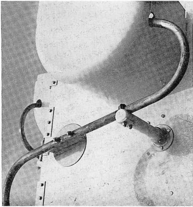
FIG. 7. Photo showing radome protective cover, radiator support and disc-shape impedance compensating capacitor.
