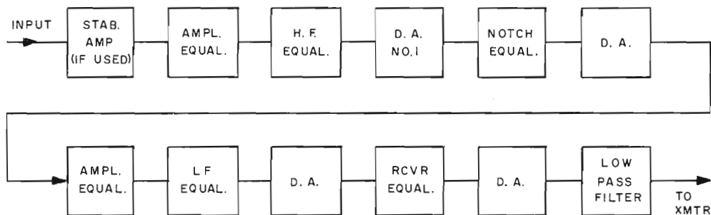
FIG. 2. Block diagram showing proper lineup of equalizers and distribution amplifiers. If stretch is used in the Stab Amp, the unit should be placed after the phase equalizers rather than as shown.
