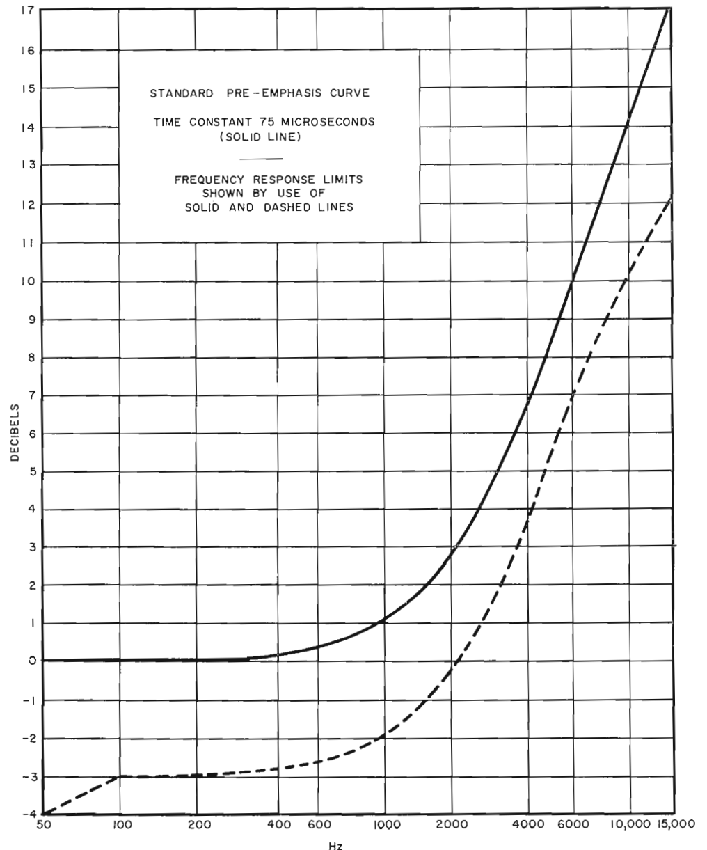
FIG. 26. Standard audio pre-emphasis curve.
