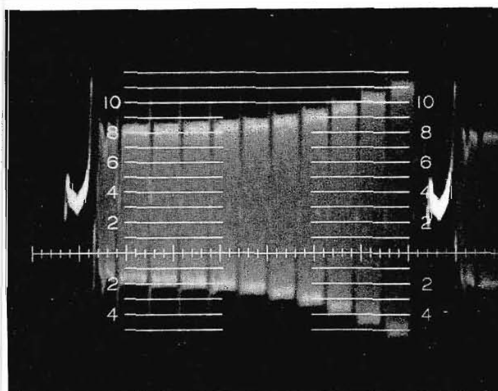
(j) Modulator output — predistorted (differential gain).
