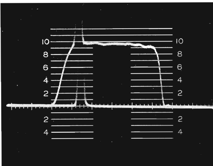
(h) Output of filterplexer.
