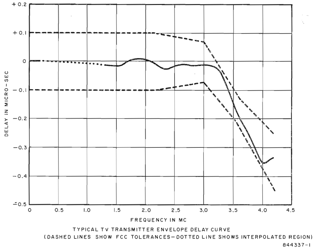
FIG. 20. Curves showing typical envelope delay characteristics as specified by FCC.
