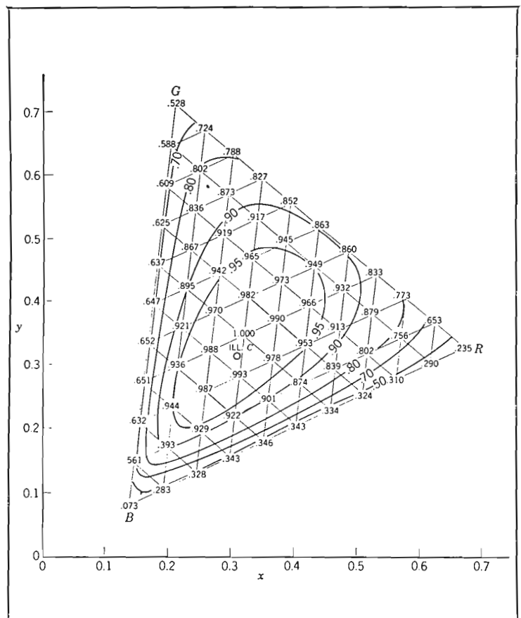
FIG. 5. Chart showing ratio (Y')^\gamma / Y of the luminance produced by the RGB camera (Y')^\gamma = rR^{1/\gamma} + gG^{1/\gamma} + bB^{1/\gamma} to the correct luminance (Y^{1/\gamma})^\gamma = Y .
