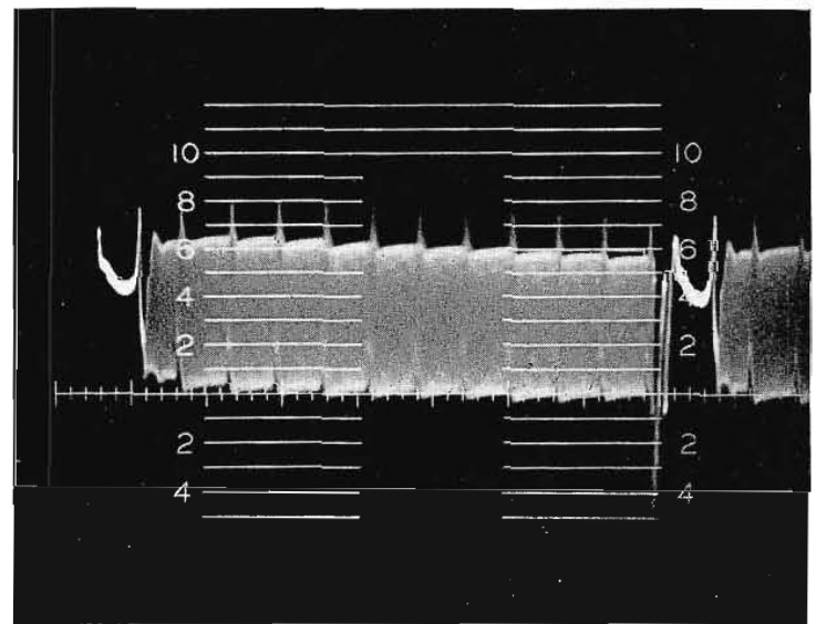
(k) Overall differential gain (differential phase 2.5°).
