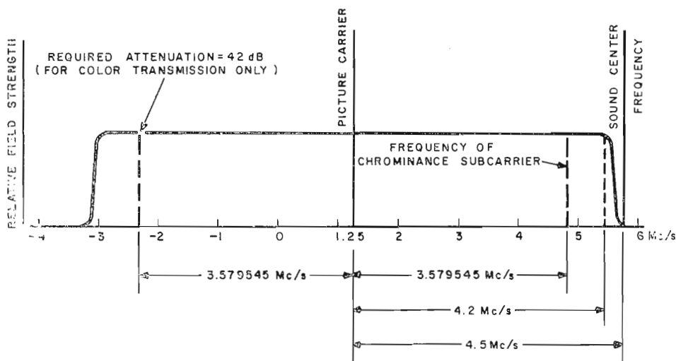
FIG. 8. Idealized double sideband picture transmission amplitude characteristic.
