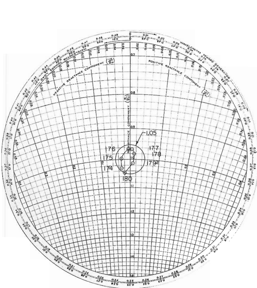
FIG. 10. Smith chart of input impedance for the Zee Panel antenna.
