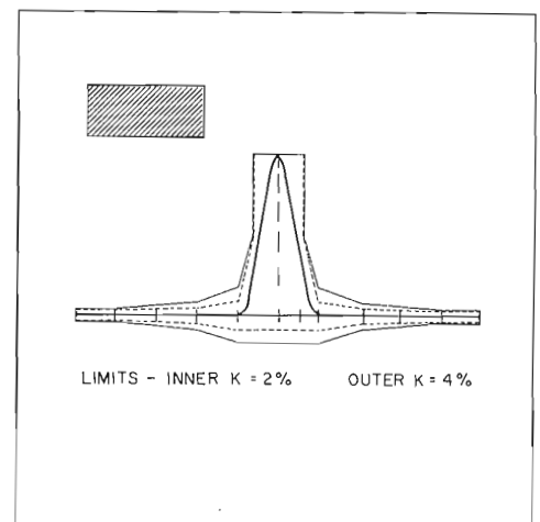
FIG. 25. Limits for 2T pulse response.
