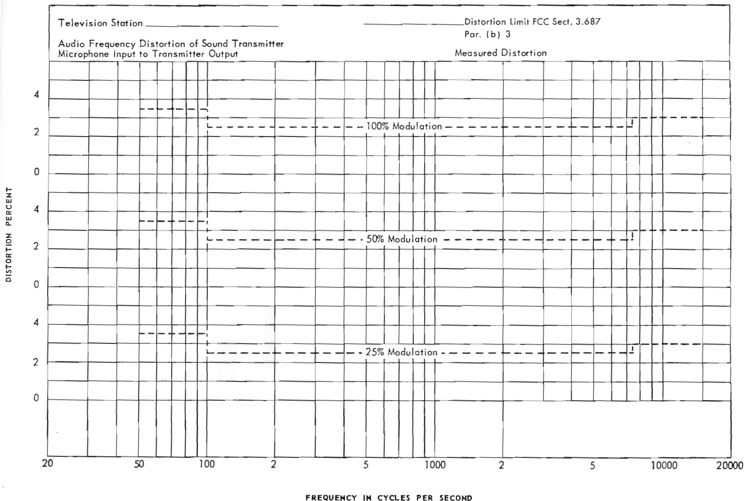
FIG. 27. Audio frequency distortion limits.
