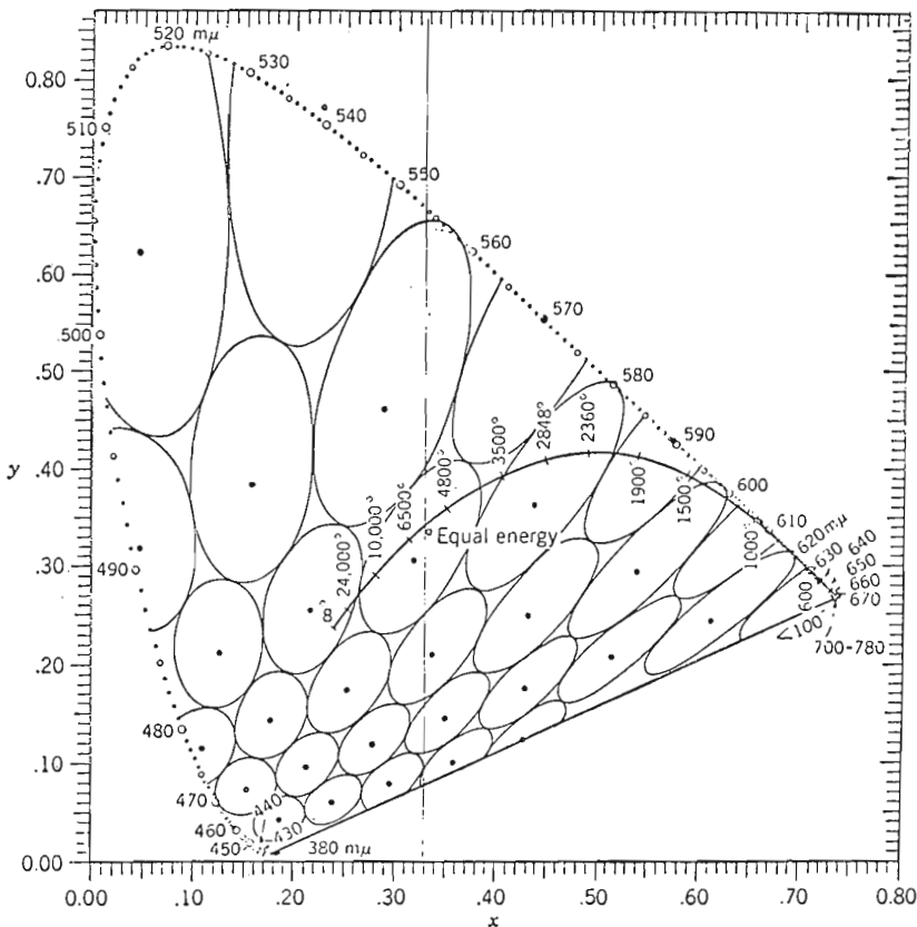
FIG. B2. MacAdams Ellipses showing Approximate Perceptibility of Chromaticity Differences in the xy chromaticity diagram. Each closed curve shows 100 times the JPCD under moderately good viewing conditions.
